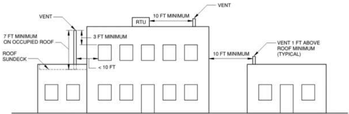
Vent minimum distances. (Figure by L. Kayo)
