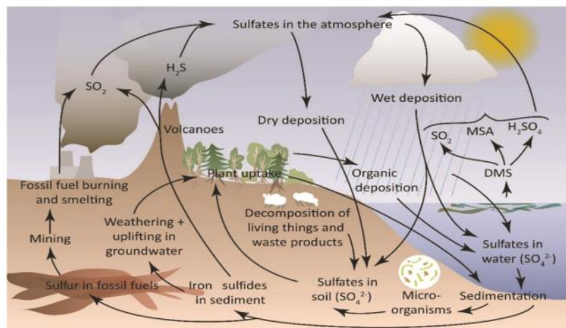
The Sulfur Cycle (source: Wikimedia)
